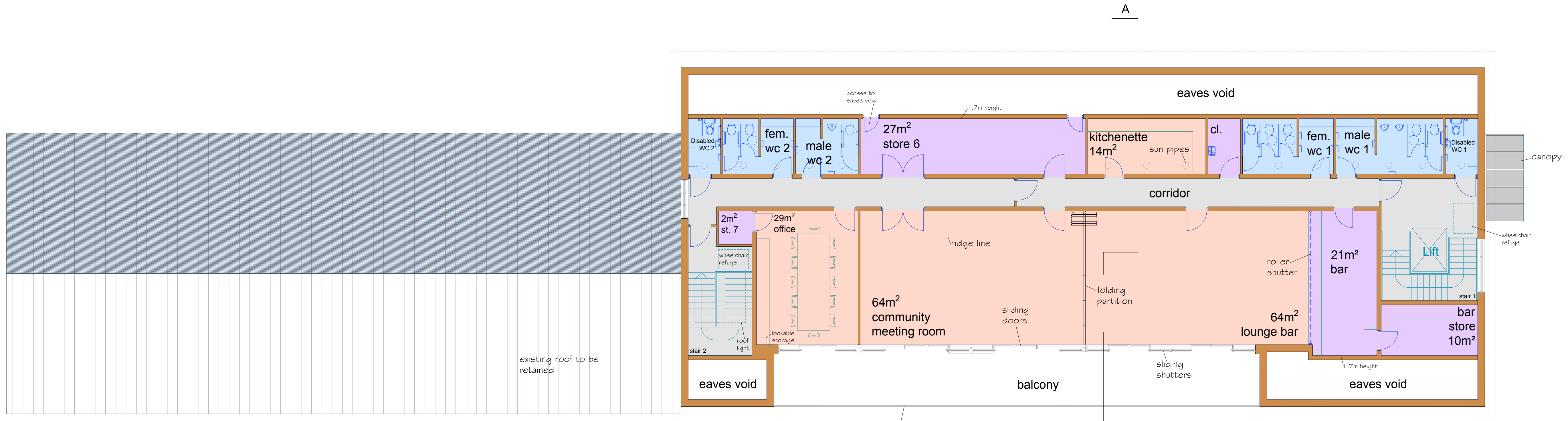
FIRST FLOOR PLAN gross internal floor area = 386.79m 2
